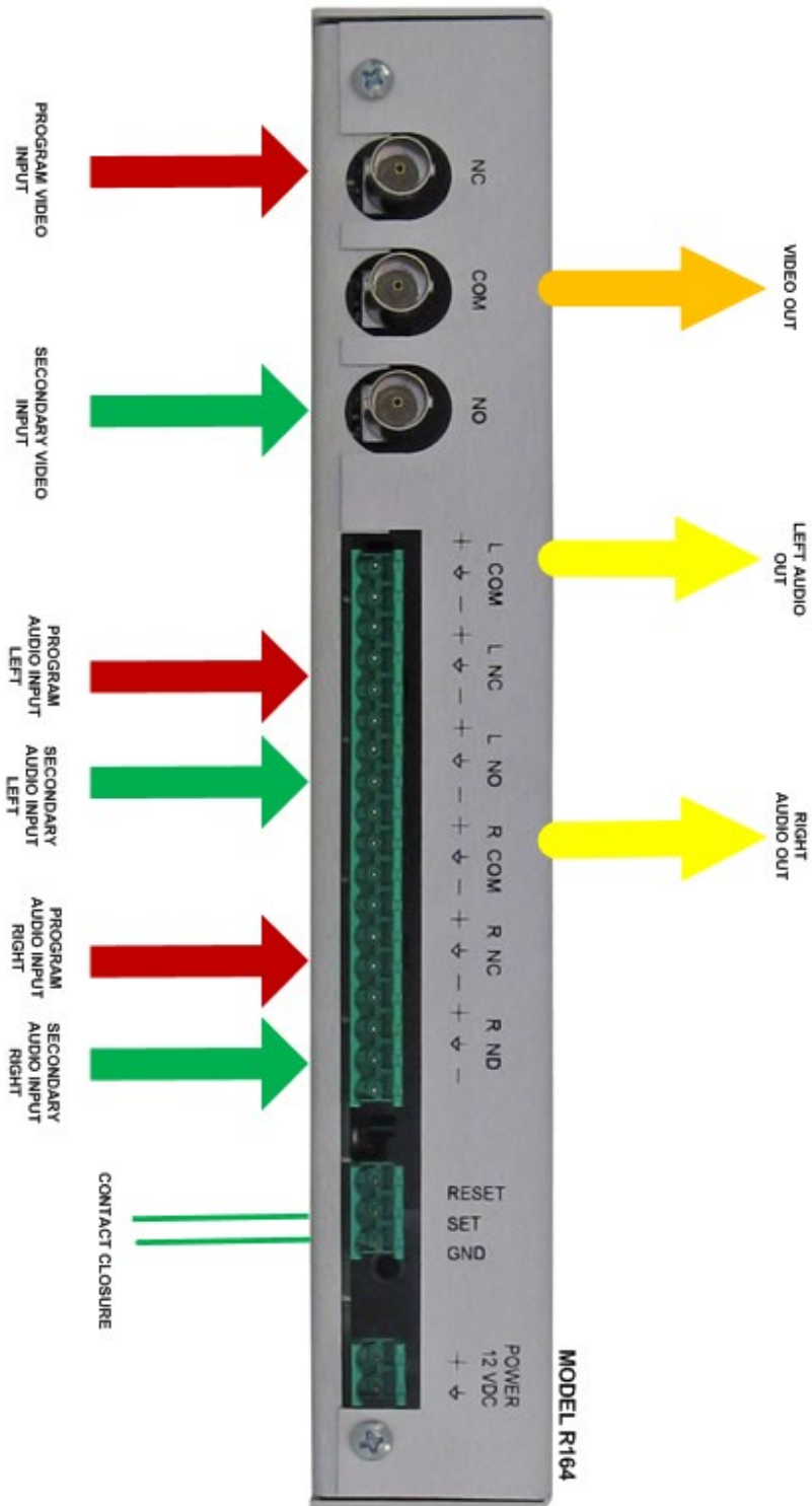
R164 CONNECTION DIAGRAM
